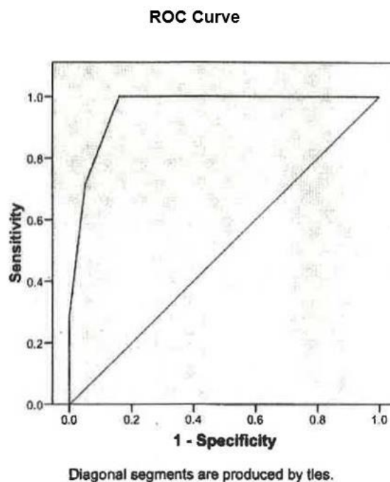
Figure 9: ROC curve
